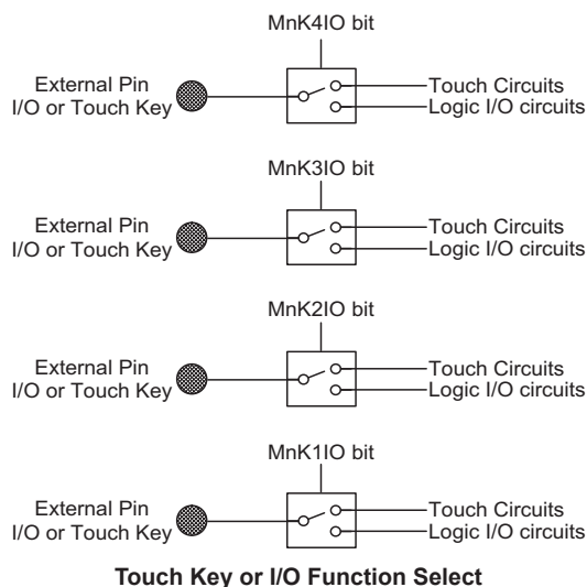
Touch Switch Module Block Diagram
